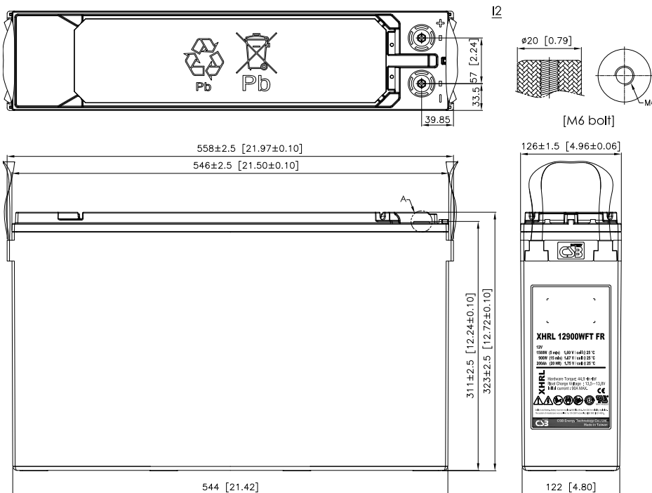
Detail A Drawing(4:1)
