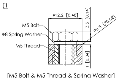
Detail A Drawing(4:1)
