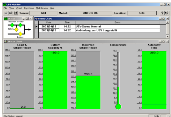
Windows UPSMON/UPSVIEW Monitoring a simple Network UPS
